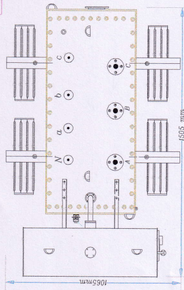
Top View Dimension
